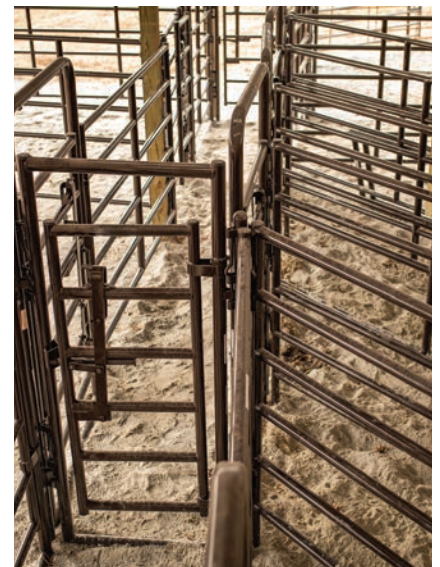
Pass-through panels feature heavy-duty double-latch.
